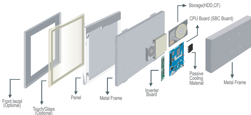
Modularized Construction
