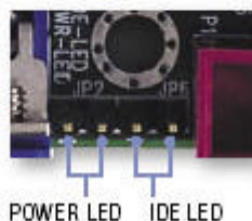
Reserved Pin Connector for additional Power/IDE LED
