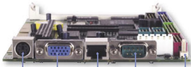
PS/2 KB/Mouse VGA Connector 10Mbps Ethernet COM1 RS-232 COM2 RS-485
