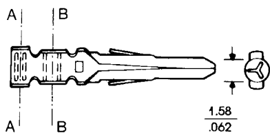
TERMINAL MACHO
